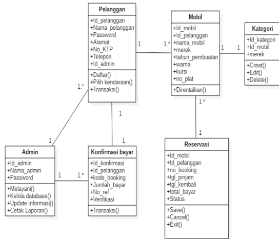
Gambar 14. Class Diagram
