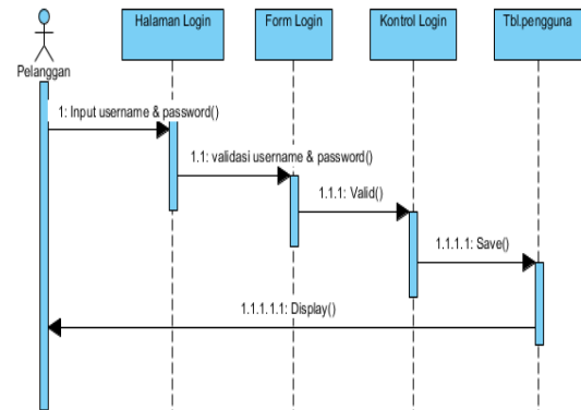
Gambar 12. Sequence Digram Login
